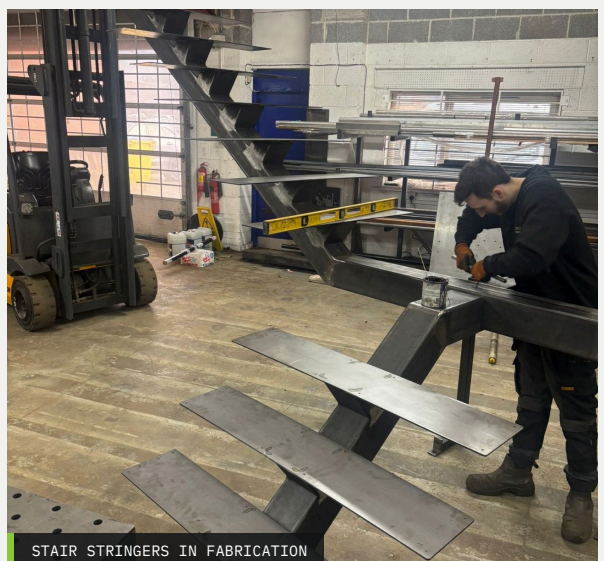
STAIR STRINGERS IN FABRICATION
